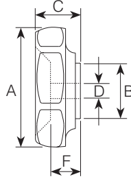
Phenolic Square Through Hole
