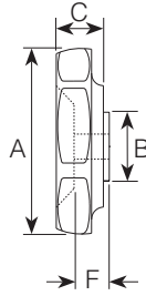
Phenolic Through Hole
